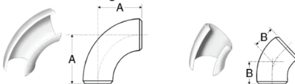
Dimensions (based on ASME/ANSI B16.9) and example weights for long radius elbows
